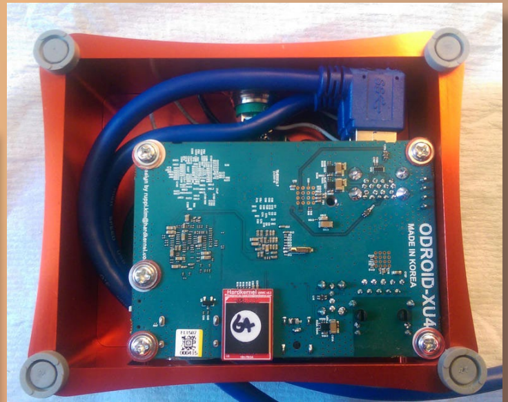
Figure 9 - Final assembly of the case with the bottom removed
