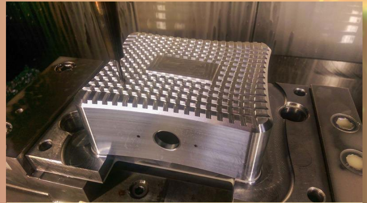
Figure 3 - Creating the cooler fins on the top outside of the case
