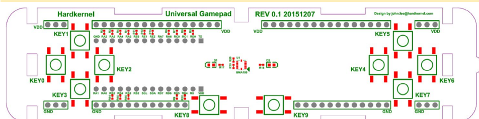
Figure 9 - Joypad PCB diagram
