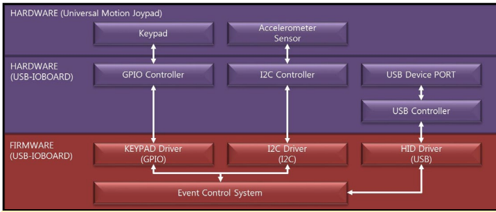
Figure 4 - Joypad Interface Diagram
