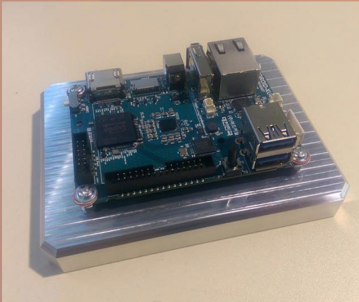
Figure 1 - ODROID-XU4 attached to the base
