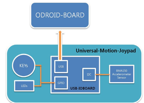
Figure 3 - Joypad Block Diagram
