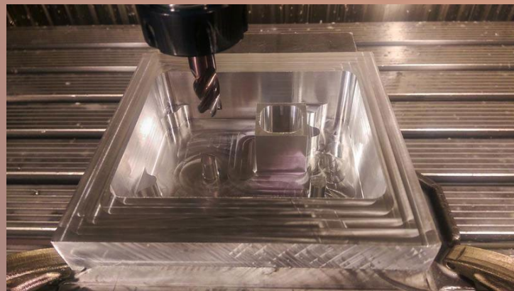
Figure 2 - Milling the top inside part of the case
