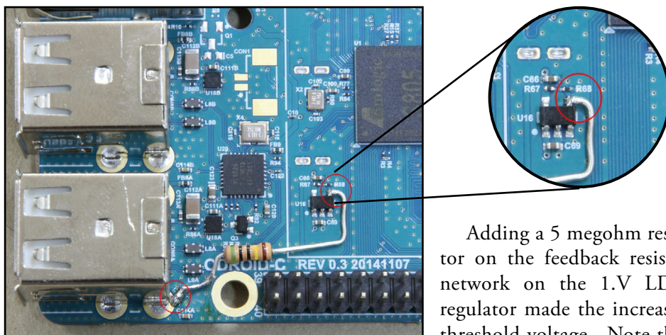
Adjusting the VDDIO with a resistor
