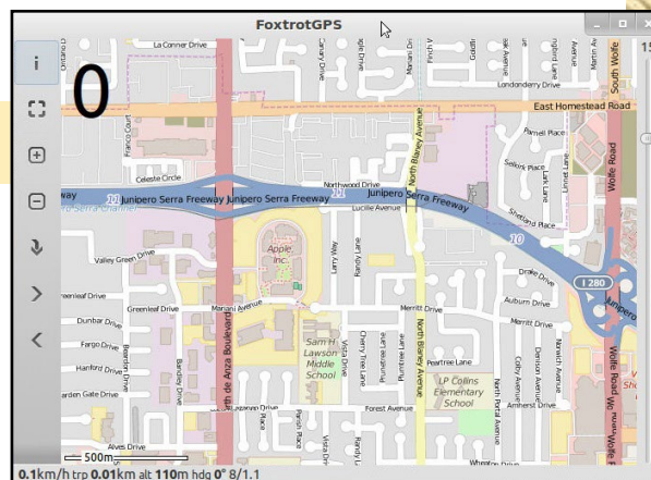
Figure 2: FoxTrotGPS UI
