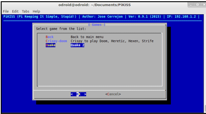
Figure 5 - PiKISS Shareware
